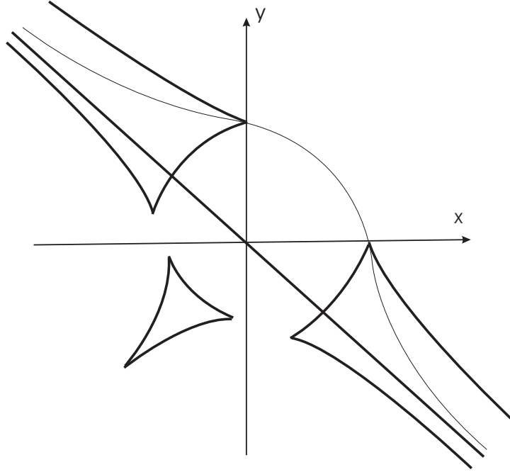
FIGURE 3. Symmetry defect set for elliptic curve x^3 + y^3 = 1 .
