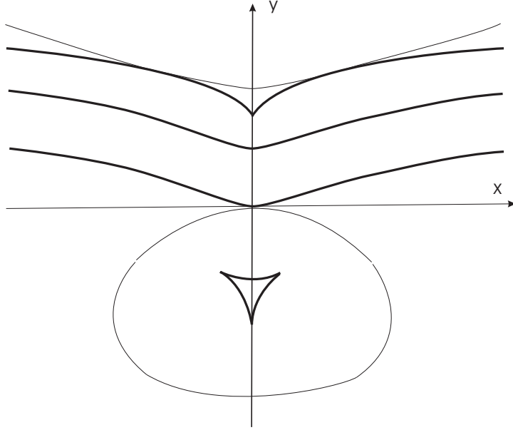
FIGURE 4. Symmetry defect set for elliptic curve x^2 = y^3 - y .
