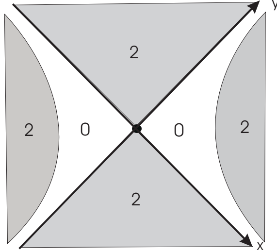
FIGURE 1. Symmetry defect set for hyperbola
