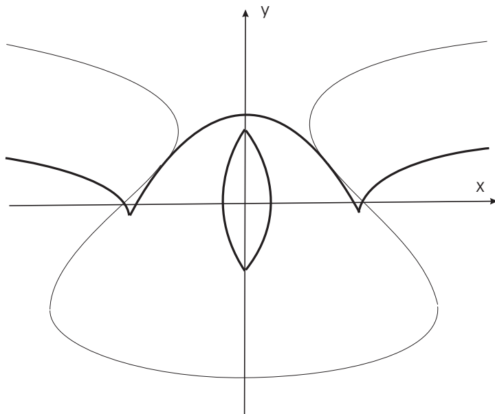
FIGURE 5. Symmetry defect set for elliptic curve y^2 = x^3 - x + 1 .
